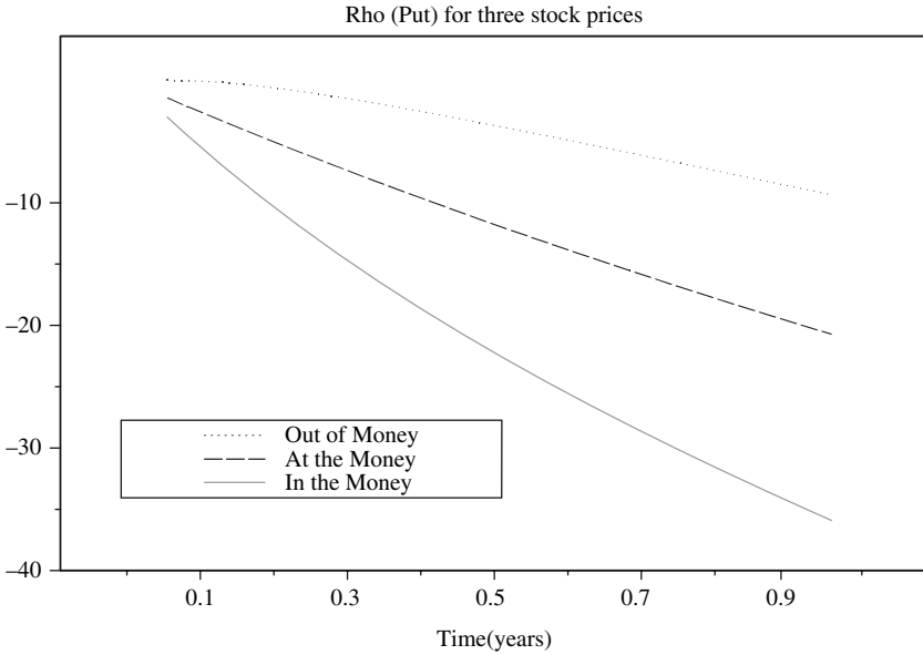
FIGURE 10.16. Rho put.
