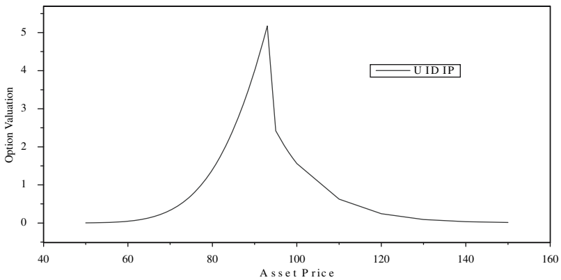
FIGURE 18.7B. UIDIP discontinuity.
