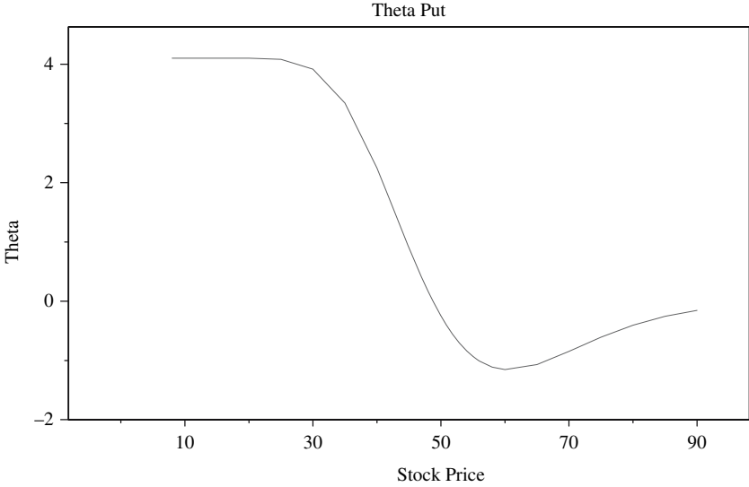
FIGURE 10.8. Theta Put.
