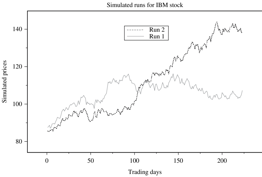
FIGURE 7.8. Simulated series.
