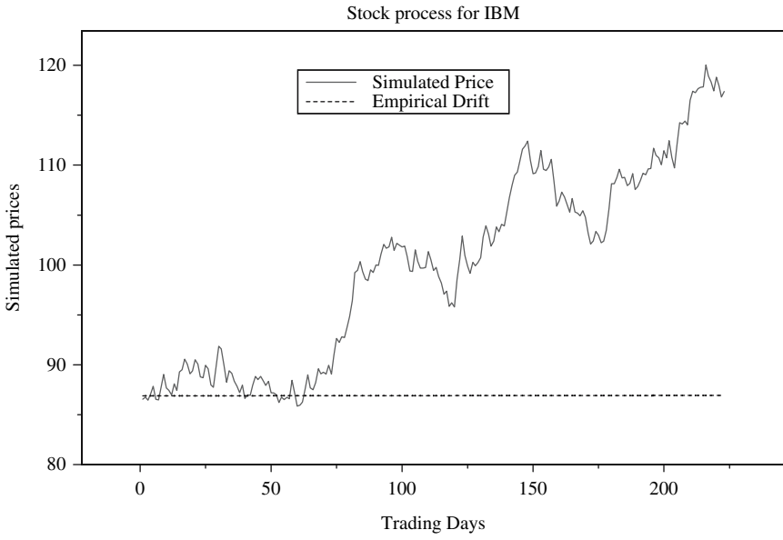
FIGURE 7.7. Price simulation.
